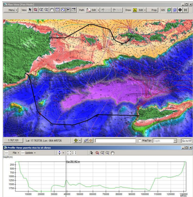
A screenshot of MakaiPlan showing the plan and profile views for a cable route near Puerto Rico.
